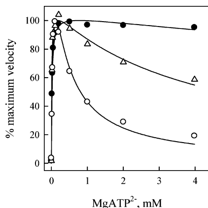
FIGURE 5: Effect of free \text{Mg}^{2+} and fructose-6-P on the \text{MgATP}^{2-} -induced inhibition of wild-type Pfk-2. Activity measurements were done at 0.1 mM fructose-6-P in the presence of 1 mM (○) and 30 mM (△) free \text{Mg}^{2+} and at 1 mM fructose-6-P in the presence of 1 mM free \text{Mg}^{2+} (●). Results are expressed as percent of enzymatic activity referred to the maximum value obtained for each condition.
