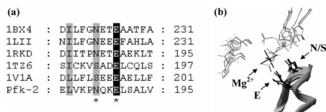
FIGURE 1: (a) Sequence alignment obtained from the structural superposition of crystallographic structures of adenosine kinases from H. sapiens (1bx4) and T. gondii (1lii), ribokinase from E. coli (1rkd), AIR kinase from S. enterica (1tz6), and 2-keto-3-deoxygluconate kinase from T. thermophilus (1v1a) and the sequence of Pfk-2 from E. coli . Conserved and identical residues are highlighted in gray and black, respectively. N/S and E from the NXXE motif are marked with an asterisk. (b) Structural superposition of 1bx4, 1lii, 1rkd, 1tz6, and 1v1a around the NXXE motif. Side chains of the residues marked with an asterisk in (a) are shown in black. Mg^{2+} ion from 1bx4 is also shown in black. Active site ligands are shown in light gray.
