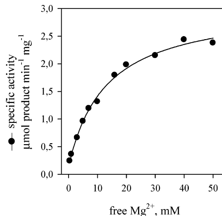
FIGURE 3: Effect of free Mg^{2+} concentration on the activity of the E190Q mutant Pfk-2. The activity of the E190Q mutant was measured as a function of the free Mg^{2+} concentration at 1 mM MgATP^{2-} and 2 mM fructose-6-P. Specific activity is expressed as \mu mol of product min^{-1} mg^{-1} .
