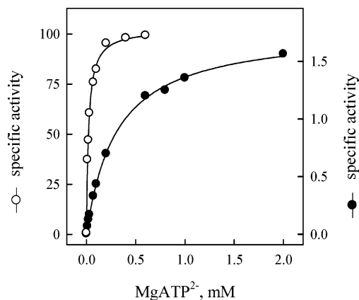
FIGURE 4: Initial velocity of wild-type and E190Q mutant Pfk-2 as a function of \text{MgATP}^{2-} concentration. The reaction velocity of wild-type Pfk-2 (○) and the E190Q mutant (●) was measured as a function of \text{MgATP}^{2-} at 30 mM free \text{Mg}^{2+} and 1 mM fructose-6-P. Specific activities are expressed as \mu\text{mol} of product \text{min}^{-1} \text{mg}^{-1} .
