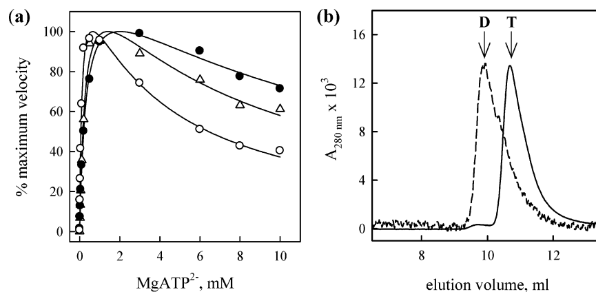
FIGURE 7: Effect of free Mg 2+ and fructose-6-P concentrations on the MgATP 2- -induced inhibition of the E190Q mutant. (a) Activity measurements were performed at 0.1 mM fructose-6-P and 1 mM free Mg 2+ (○), 0.1 mM fructose-6-P and 30 mM free Mg 2+ (△), and 1 mM fructose-6-P and 1 mM free Mg 2+ (●). (b) Elution profile from size exclusion chromatography of the E190Q mutant in the absence (---) and presence (—) of 0.2 mM MgATP 2- . T and D denote tetramer and dimer, respectively.
