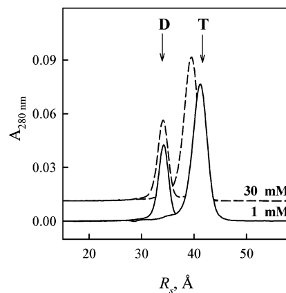
FIGURE 6: Effect of free \text{Mg}^{2+} concentration on the \text{MgATP}^{2-} -induced tetramerization of wild-type Pfk-2. The R_s of Pfk-2 was measured by size exclusion chromatography (see Experimental Procedures) in the absence (dimer) and in the presence (tetramer) of 0.1 mM \text{MgATP}^{2-} at 1 mM (—) and 30 mM free \text{Mg}^{2+} (---). Protein elution was recorded as absorbance at 280 nm. T and D denote tetramer and dimer, respectively.
