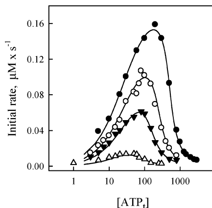
FIGURE 2: Initial velocities of the wild-type enzyme as a function of the ATP concentration at fixed Mg_i concentrations. The initial rates were obtained as a function of ATP_i with 500 \mu M (●), 250 \mu M (○), 150 \mu M (▼), and 50 \mu M (△) Mg_i . Symbols represent the experimental data while solid lines represent the simulated data obtained from the global fit to Model I ( r^2 = 0.9903 ). The r^2 value and the simulated data obtained from the global fit to Model II were very similar to those obtained from Model I (data not shown). The enzymatic assay was performed with 0.0043 \mu M wild-type Pfk-2 (in terms of monomer subunit) at 26 °C in the presence of 1 mM of fructose-6-P. The ATP_i concentration is shown in logarithmic scale of micromolar concentration to better display the data fit.
